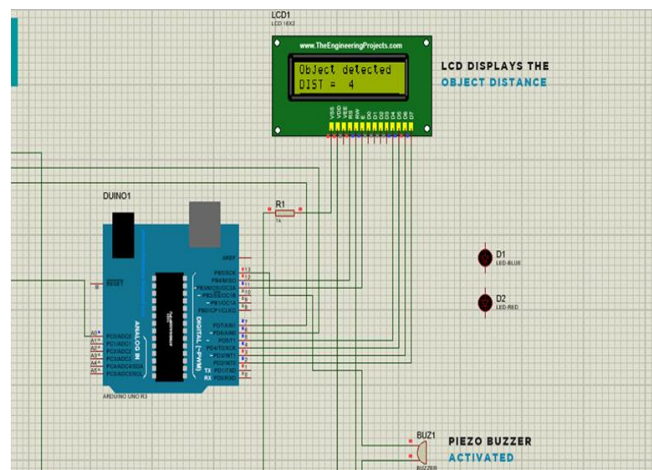
Fig 6: Displaying Object Distance Message With Buzzer Activated.
