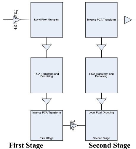
Fig 1: Denoising By Principal Component Analysis With Local Pixel Grouping (PCA-LPG)
