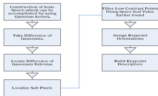
Fig 2: Diagramatic Representation of Sift Implementation
