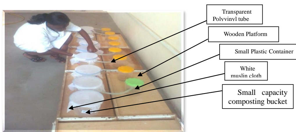
Figure 4. Laboratory Experimental Setup
