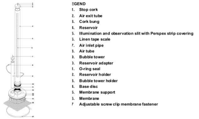
Figure 3. Isometric projection of the tension infiltrometer with the components shown in exploded view.
