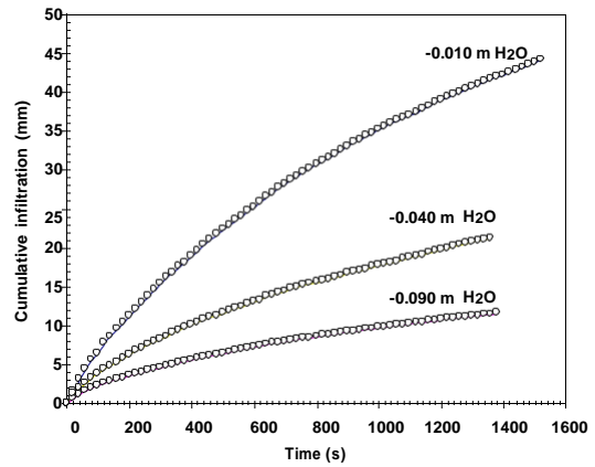
Figure 4. Typical cumulative infiltration versus time relationships obtained during infiltration tests at -0.90, 0.040 and 0.010 m H 2 O potentials.
