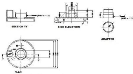
Figure 1. Details of the cast aluminium disc of the tension infiltrometer
