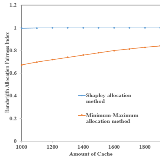
Figure 4: Bandwidth Allocation Fairness Index: Total Bandwidth = 2000Mbps, Total Bandwidth Requested = 4000Mbps, Slice number =10
