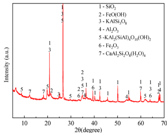
Plate 5: XRD image of Lateritic Soil
