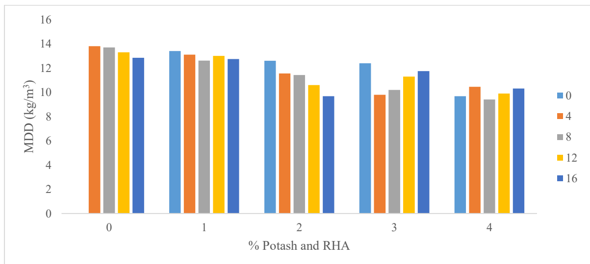
Figure 3: Maximum dry density with percentage potash and RHA chart
