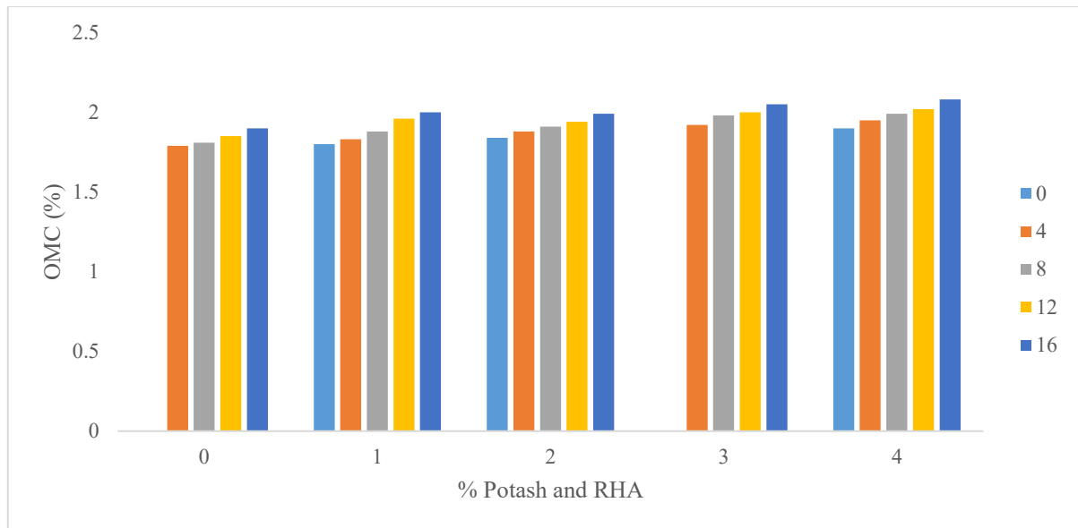
Figure 2: Optimum moisture content with percentage potash and RHA chart
