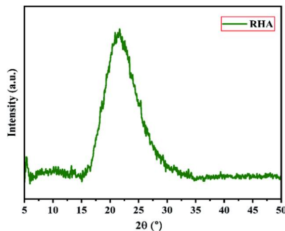
Plate 2: XRD of Rice Husk Ash (RHA)
