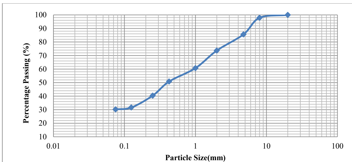
Figure 1: Graph of Sieve Analysis
