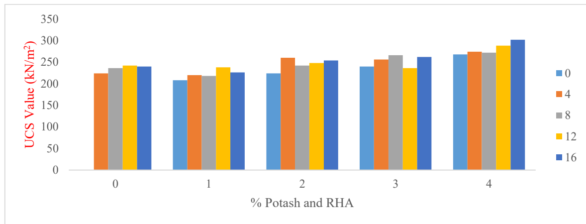
Figure 5: UCS values with percentage potash and RHA chart
