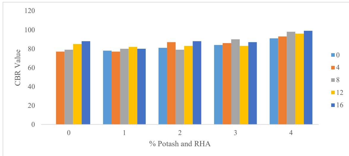
Figure 4: CBR values with percentage potash and RHA chart
