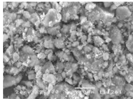
Plate 6: SEM image of Lateritic Soil
